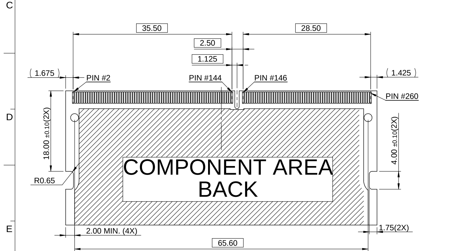
DDR4 SO DIMM MODULE BOARD LAYOUT
